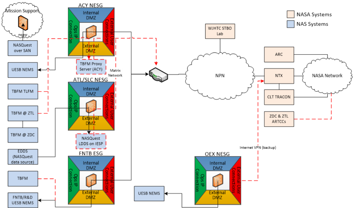
Figure 5.2 – This figure highlights the interfaces between FAA and NASA information systems for the ATD-2 field demonstration.
