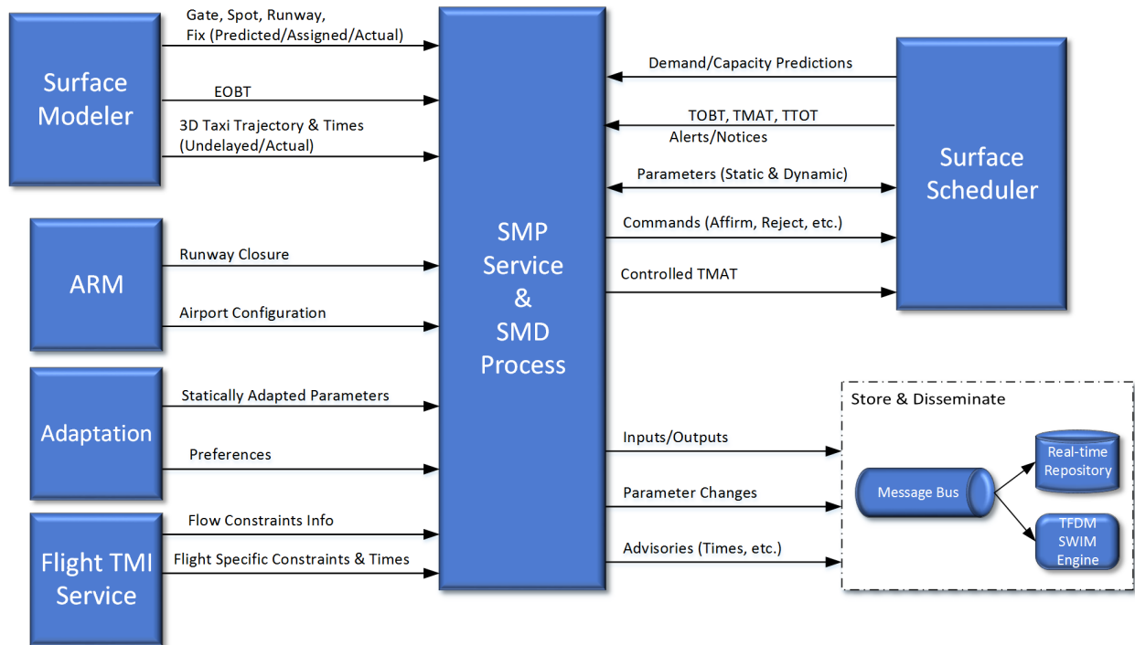
Figure 4.7 - The SMP user interface component consumes/produces a variety of data.
