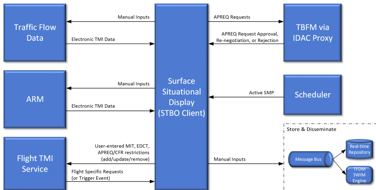
Figure 4.13 - The Surface Situational Display component consumes/produces a variety of data.
