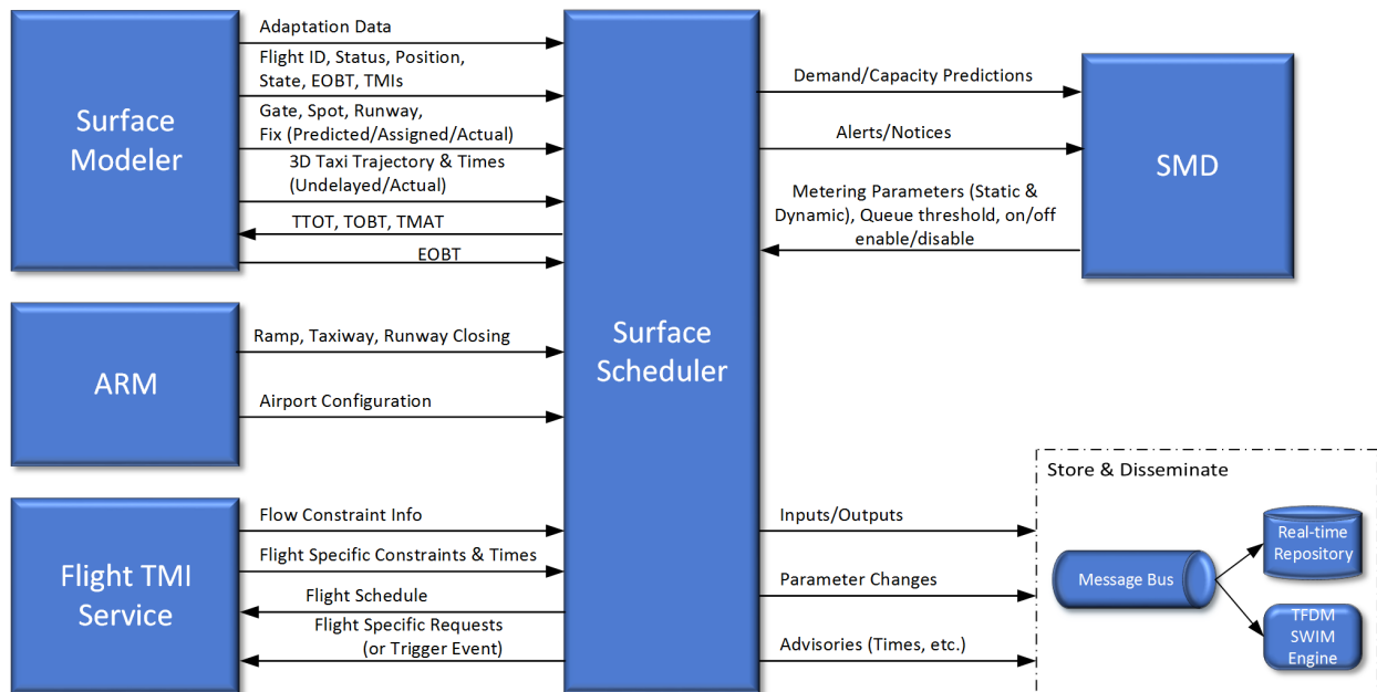
Figure 4.6 – The Surface Scheduler component consumes/produces a variety of data.
