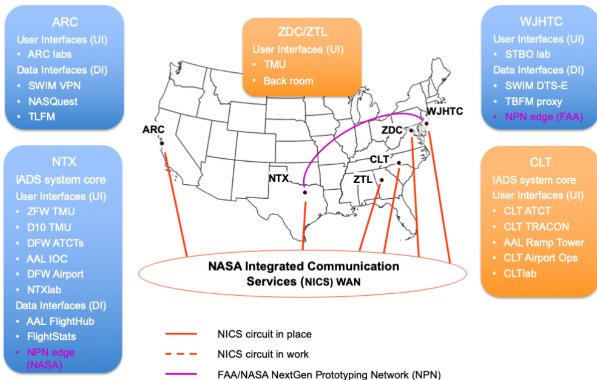
Figure 5.1 - This geographic depiction shows the locations of the NASA installations that will support the ATD-2 field demonstration.
