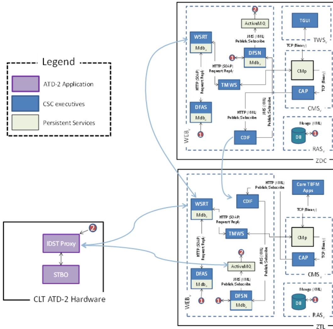
Figure 4.17 - Lockheed Martin proposes a solution leveraging TBFM-to-TBFM capability.
