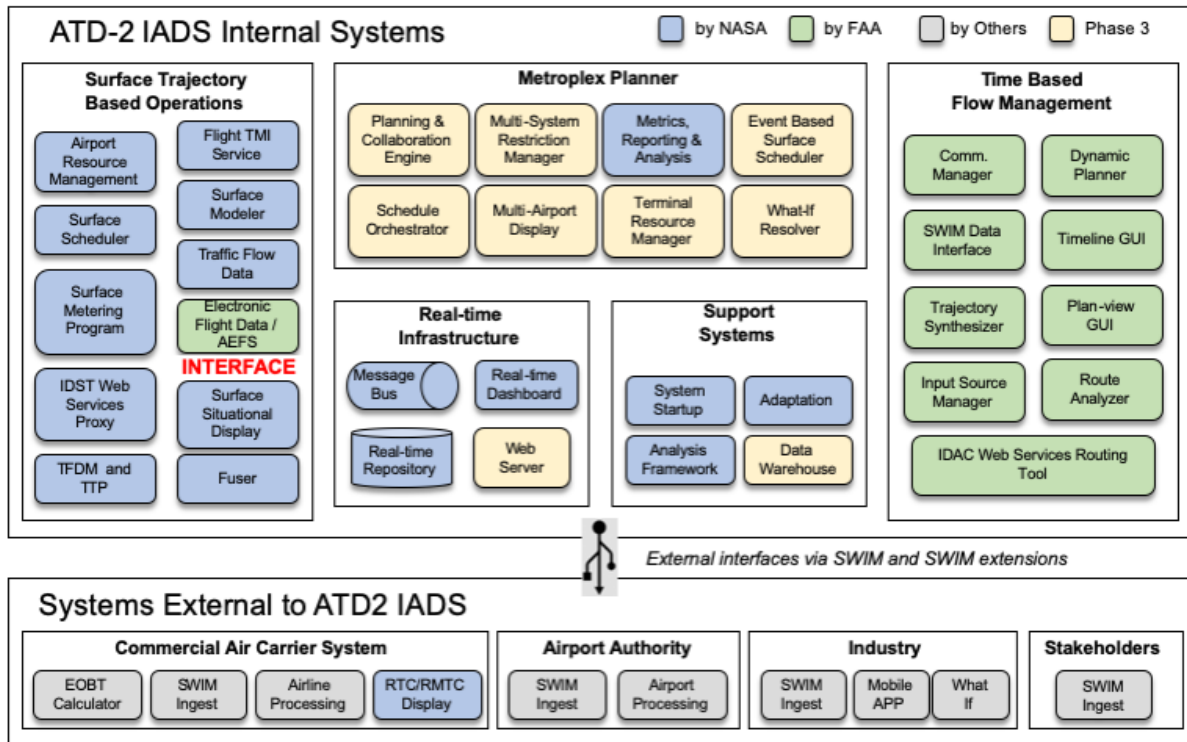
Figure 4.2 - The logical architecture for the IADS field demonstration system is shown to the next level of detail.
