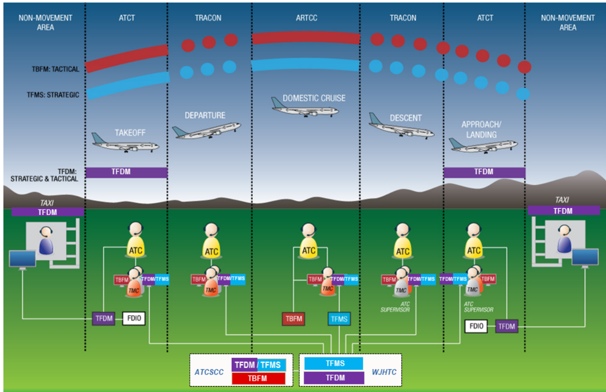
Figure 2.3 - Integrated Traffic Flow Management (TFM) systems work together to enhance the NAS [as briefed at April 2016 CDM meeting].
