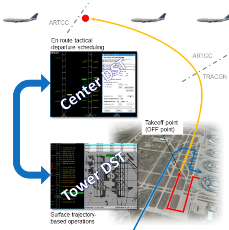
Figure 2.11 - Precision Departure Release Capability (PDRC) uses information from a trajectory-based surface system to improve TBFM tactical departure scheduling.
