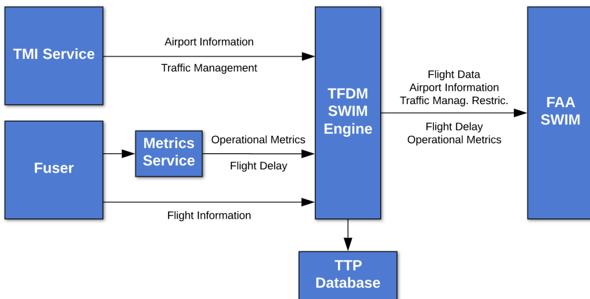
Figure 4.8 - TFDM SWIM Engine
