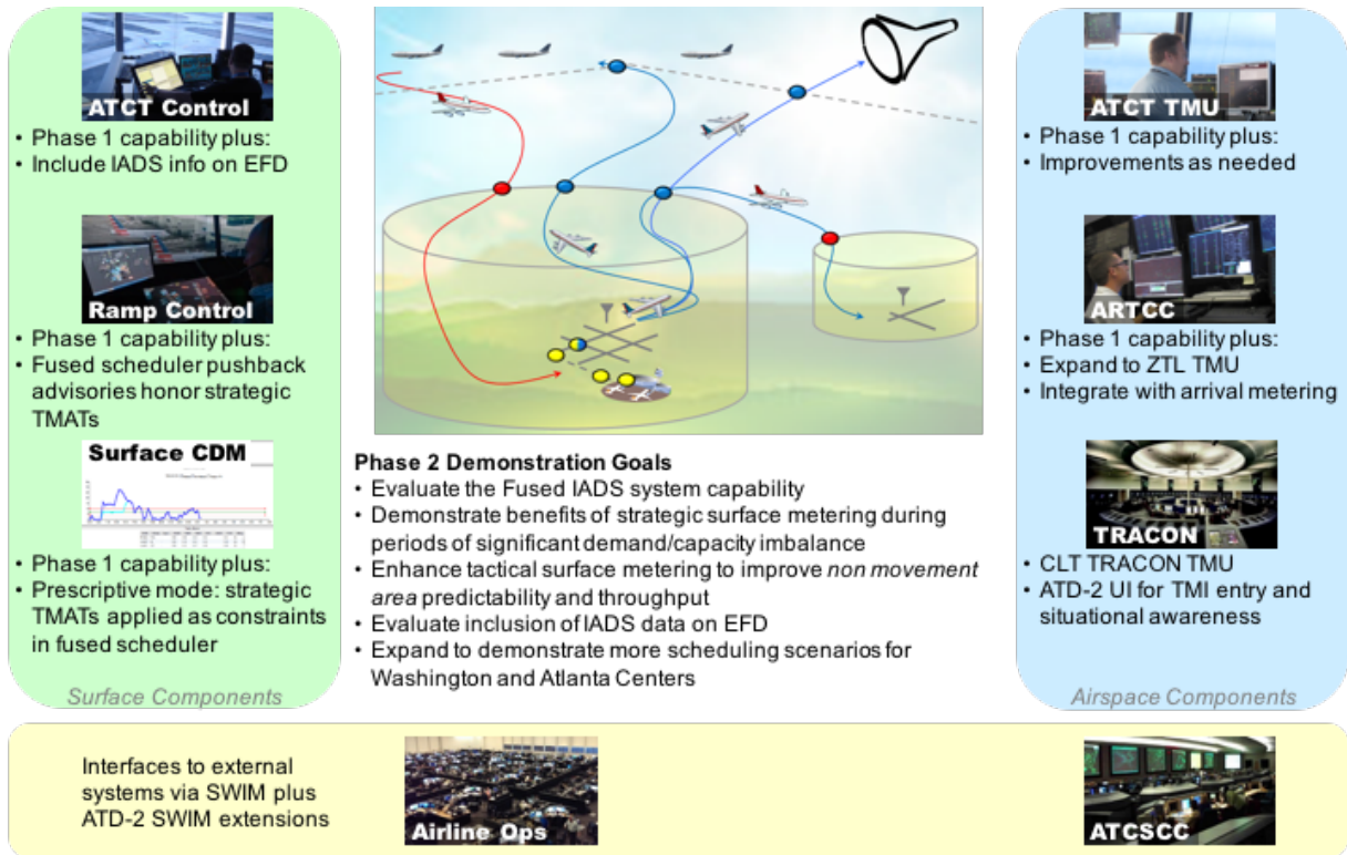
Figure B.3 - This enhanced operational overview of the IADS system highlights both the participants at various facilities and the system improvements for the Phase 2 Fused IADS Demonstration.
