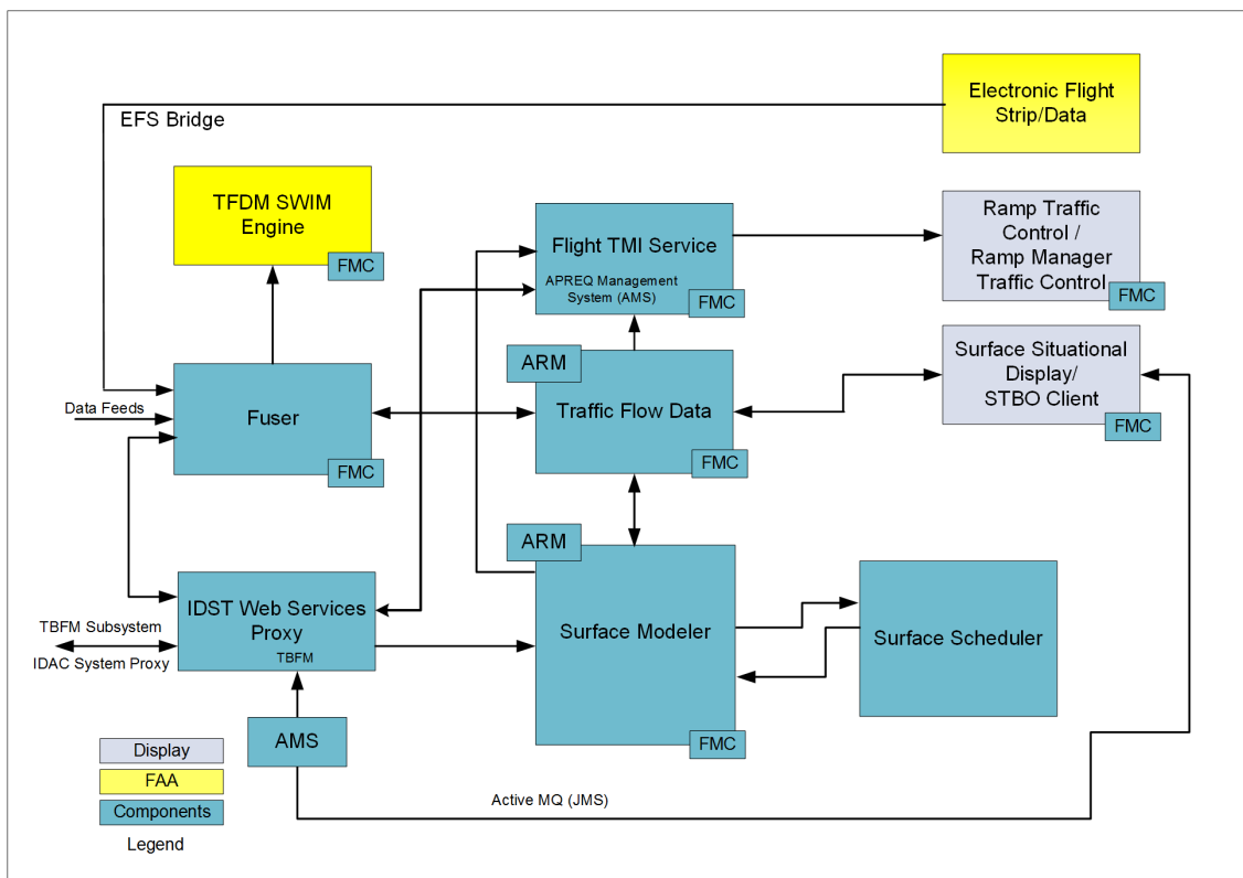
Figure 4.3 - The ATD-2 STBO Block diagram is shown as it is implemented in Phase 1.
