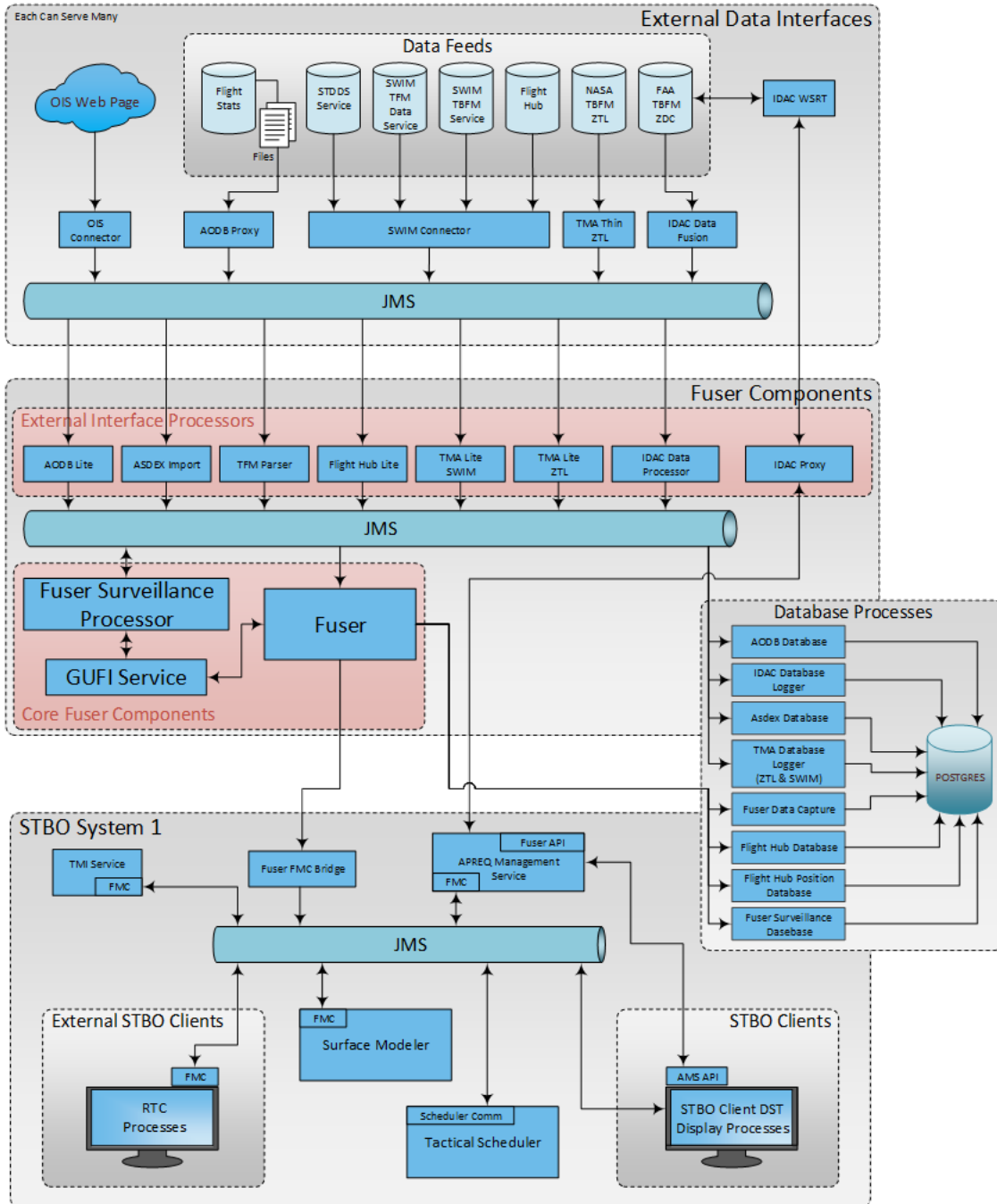
Figure 4.10 - The Fuser architecture overview shows the communication flow of the sub-components that comprise the Fuser system.
