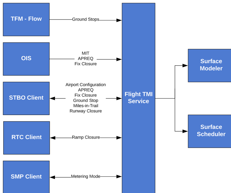
Figure 4.14 - TMI Service - Inputs/Outputs
