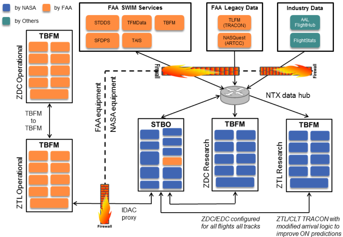
Figure 4.16 - The relationship among the TBFM and STBO systems is shown in the NASA proposed solution.
