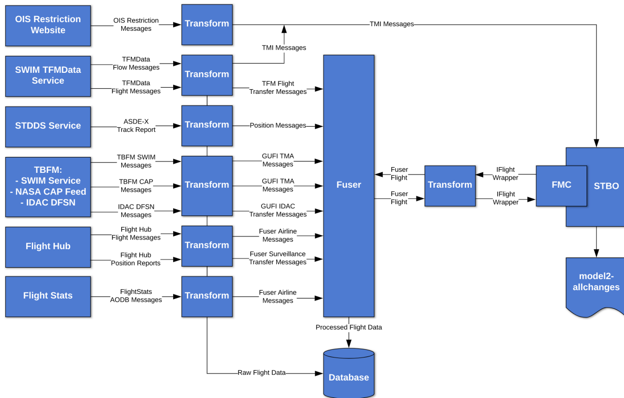
Figure 4.9 - This illustration shows the data flow to/from the Fuser.
