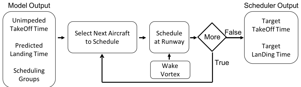
Figure 4.5 – High level design of the IADS scheduler
