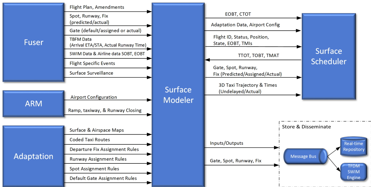
Figure 4.4 – The ATD-2 Surface Modeler component consumes/produces a variety of data.
