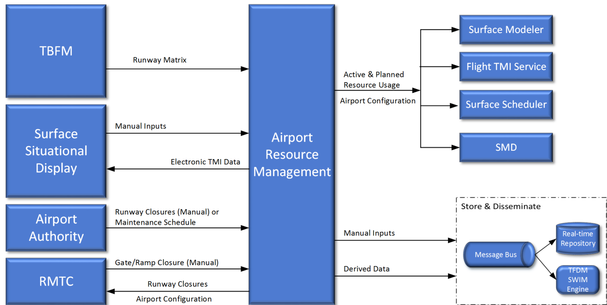
Figure 4.11 - The Airport Resource Management component consumes/produces a variety of data.
